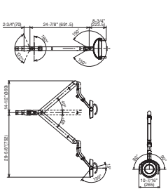
■ Unit Mount
