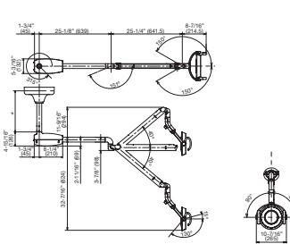
■ Ceiling Mount
