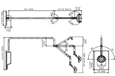
■ Wall Mount
